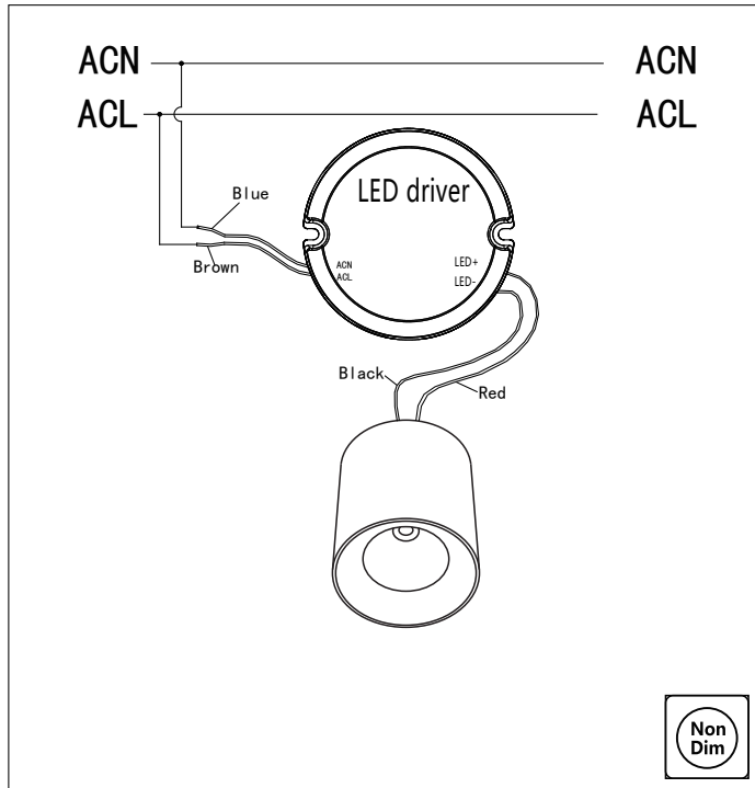
ON/OFF Wiring
